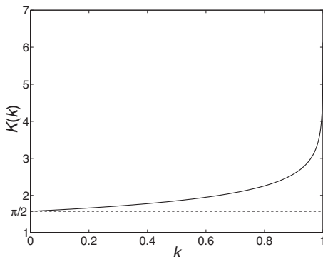
Fig. 2. The complete elliptic integral of the first kind. The function has a global minimum of \pi/2 at k=0 ( \theta_0=0^\circ ) and monotonically increases to infinity at k=1 ( \theta_0=180^\circ ). The dashed line corresponds to the small-angle approximation K(k)=\pi/2 .
