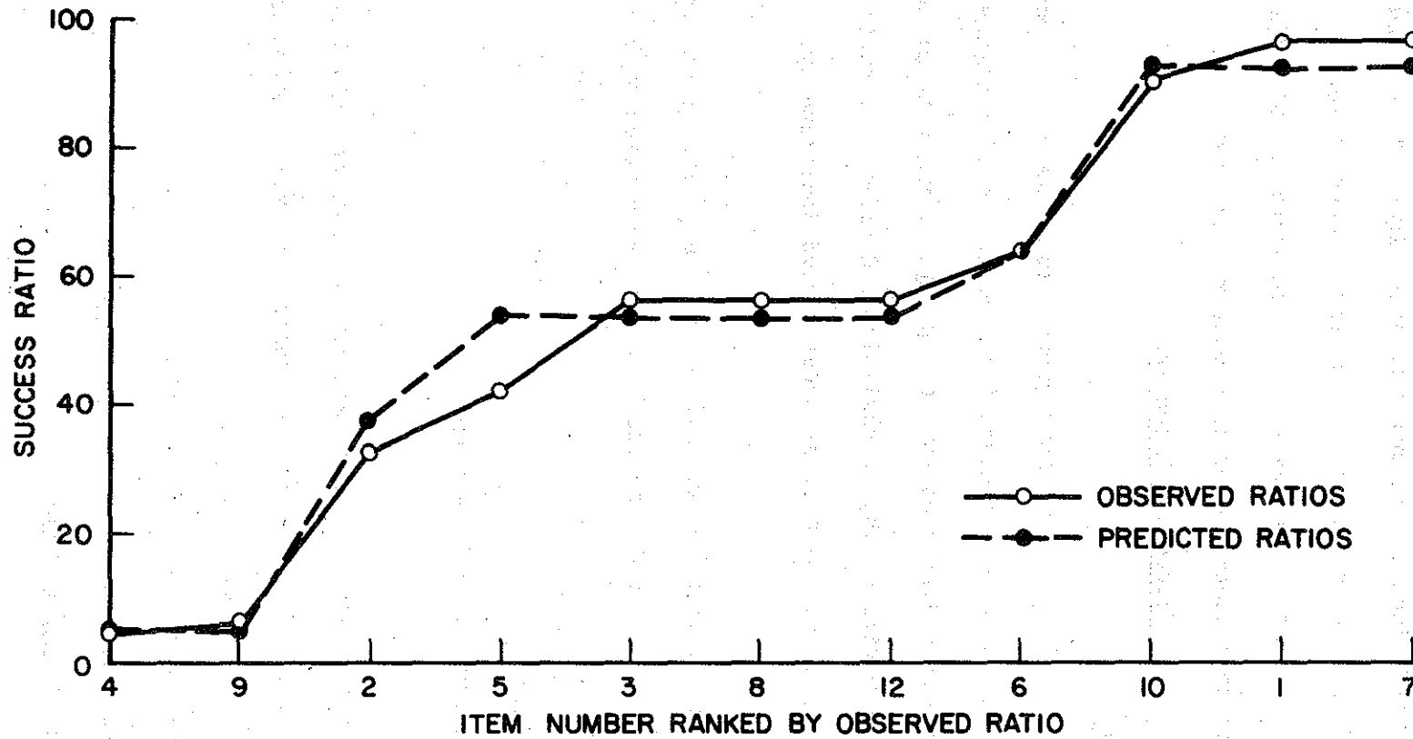
Figure 2. Predicted and observed success ratios with four variables in the regression equation, Experiment 1.
