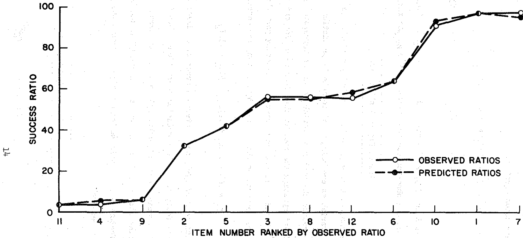
Figure 1. Predicted and observed success ratios with eight variables in the regression equation, Experiment 1.
