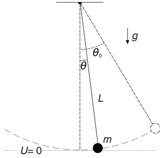
Fig. 1. A simple pendulum of mass m and length L oscillating in a vertical plane. The particle is displaced to the angle \theta_0 and then released at rest. The system oscillates under the action of gravity. The angular displacement \theta is measured counter-clockwise relative to the equilibrium position ( \theta=0 ).
