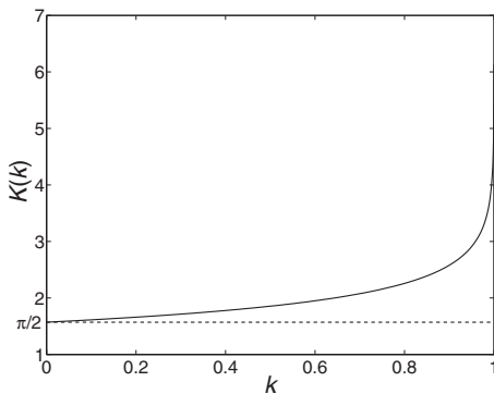
Fig. 2. The complete elliptic integral of the first kind. The function has a global minimum of \pi/2 at k=0 ( \theta_0=0^\circ ) and monotonically increases to infinity at k=1 ( \theta_0=180^\circ ). The dashed line corresponds to the small-angle approximation K(k)=\pi/2 .
